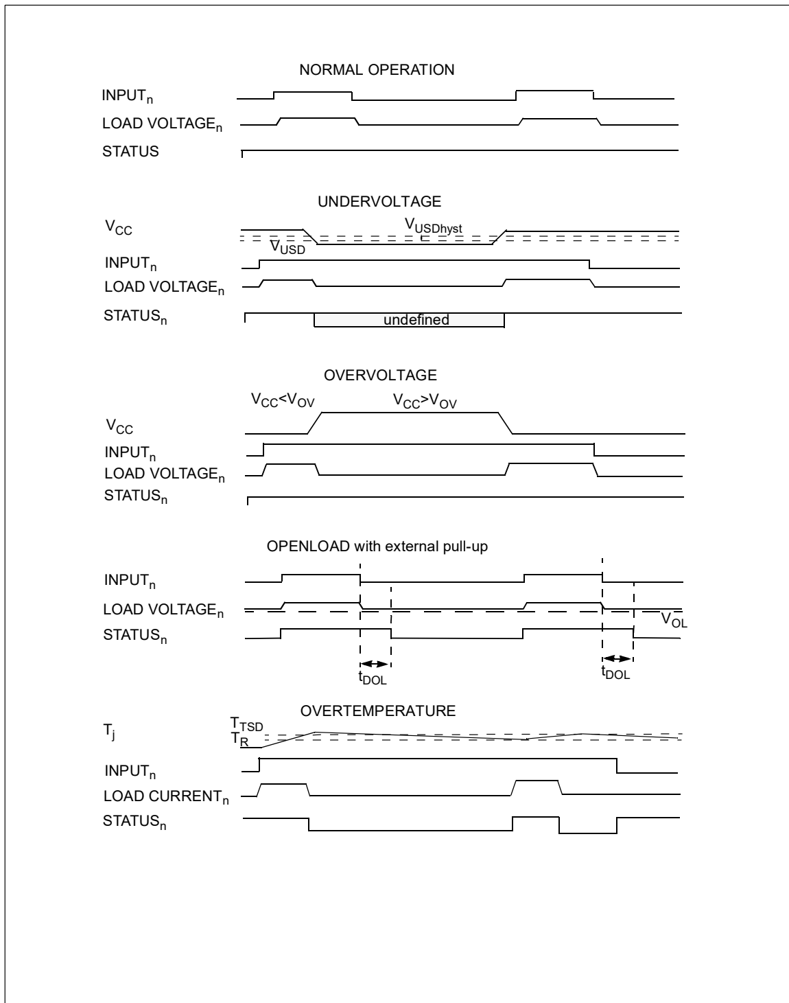
Figure 2: Waveforms
